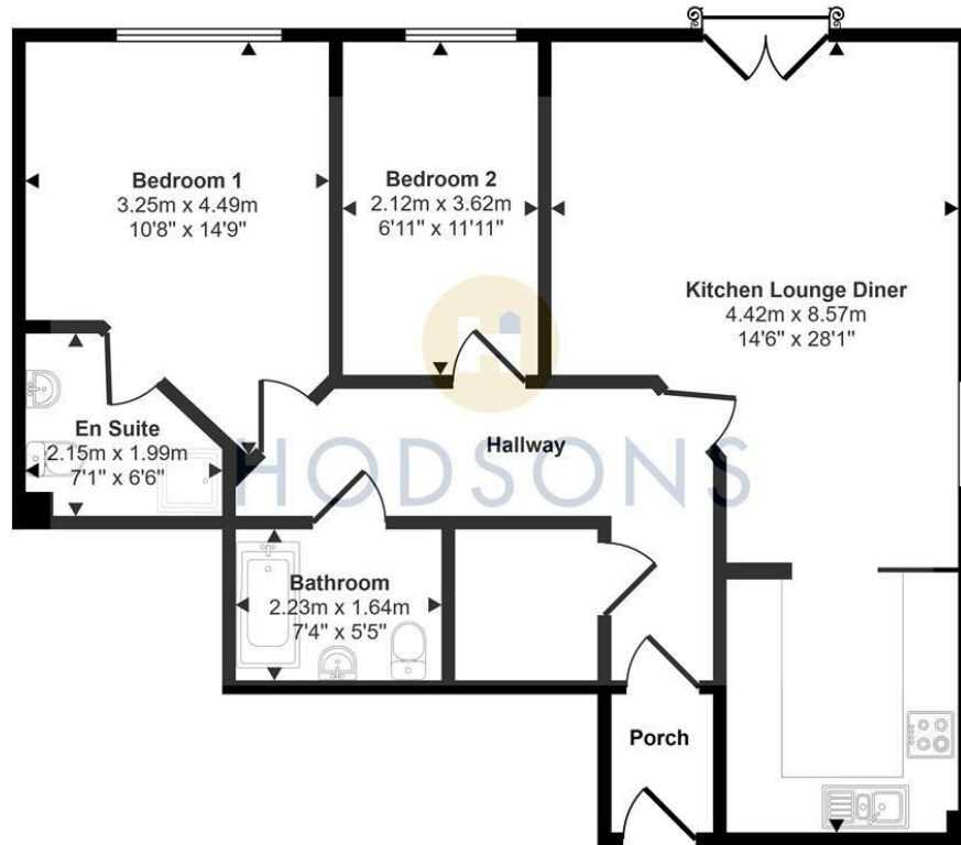
Floorplan
